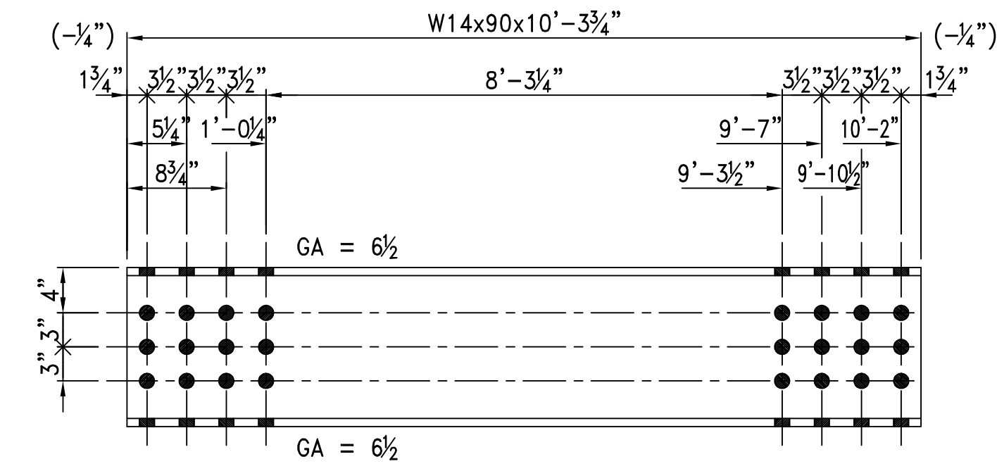
16 - BEAM - 3B1
