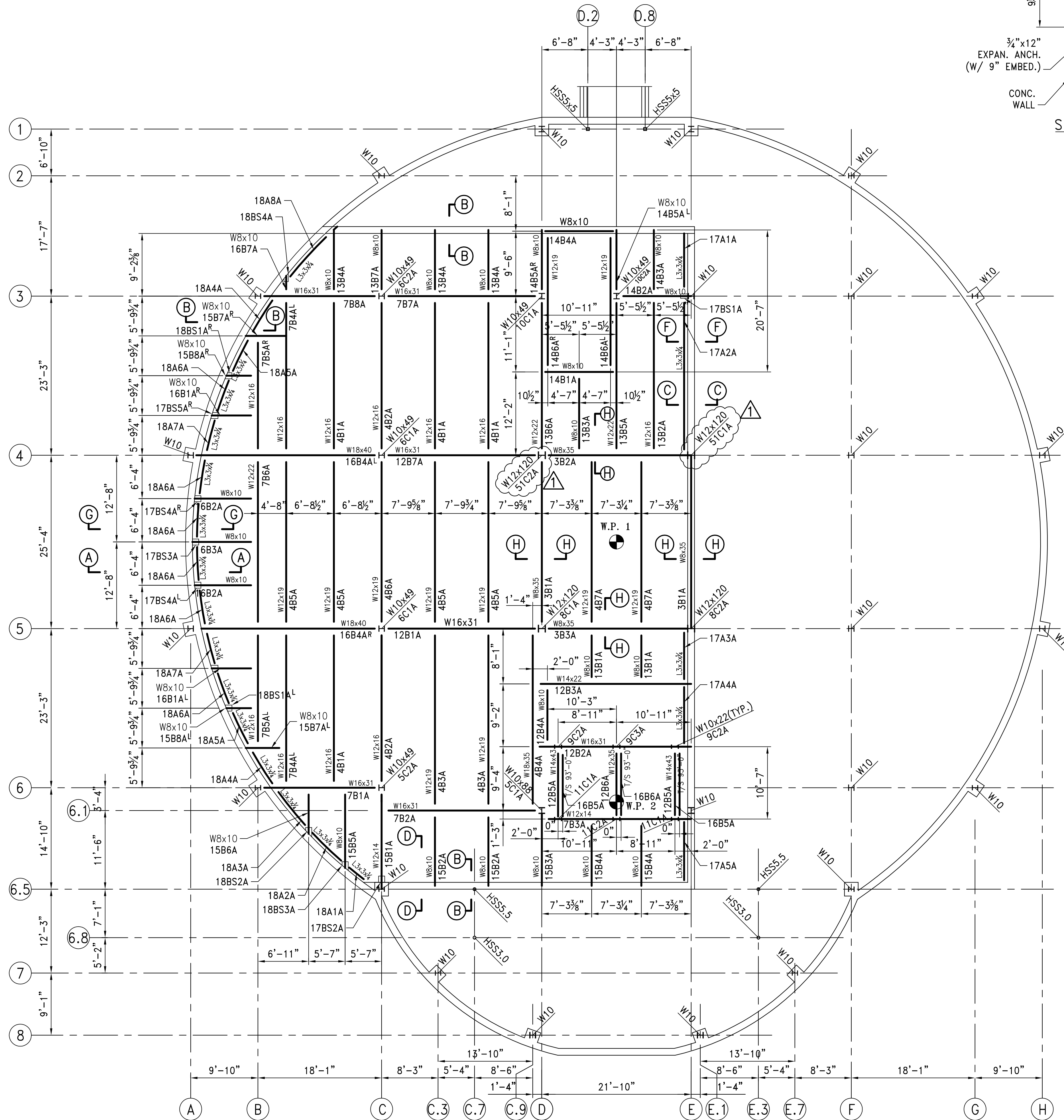
1st FLOOR FRAMING PLAN T/STL EL. 99'-8" U.N.
